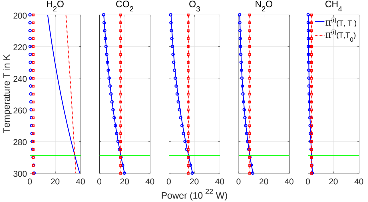
Figure 23: The continuous blue lines are the powers \Pi^{\{i\}}(T, T) of (111), emitted by a single greenhouse-gas molecule at the temperature T . The dotted red lines are the powers \Pi^{\{i\}}(T, T_0) of (110) absorbed by a single greenhouse molecule at the temperature T from thermal-equilibrium radiation at the temperature T_0 = 288.7 K, shown by the horizontal green line. The blue circles and red squares are the analogous powers from the harmonic oscillator approximation of (148), summed for all vibrational modes of the molecule shown in Table 8 of the Appendix. The emitted and absorbed powers are well modeled with harmonic oscillators for all gases except for the asymmetric-top molecule, H 2 O, where most of the power is emitted and absorbed by pure-rotation transitions.
