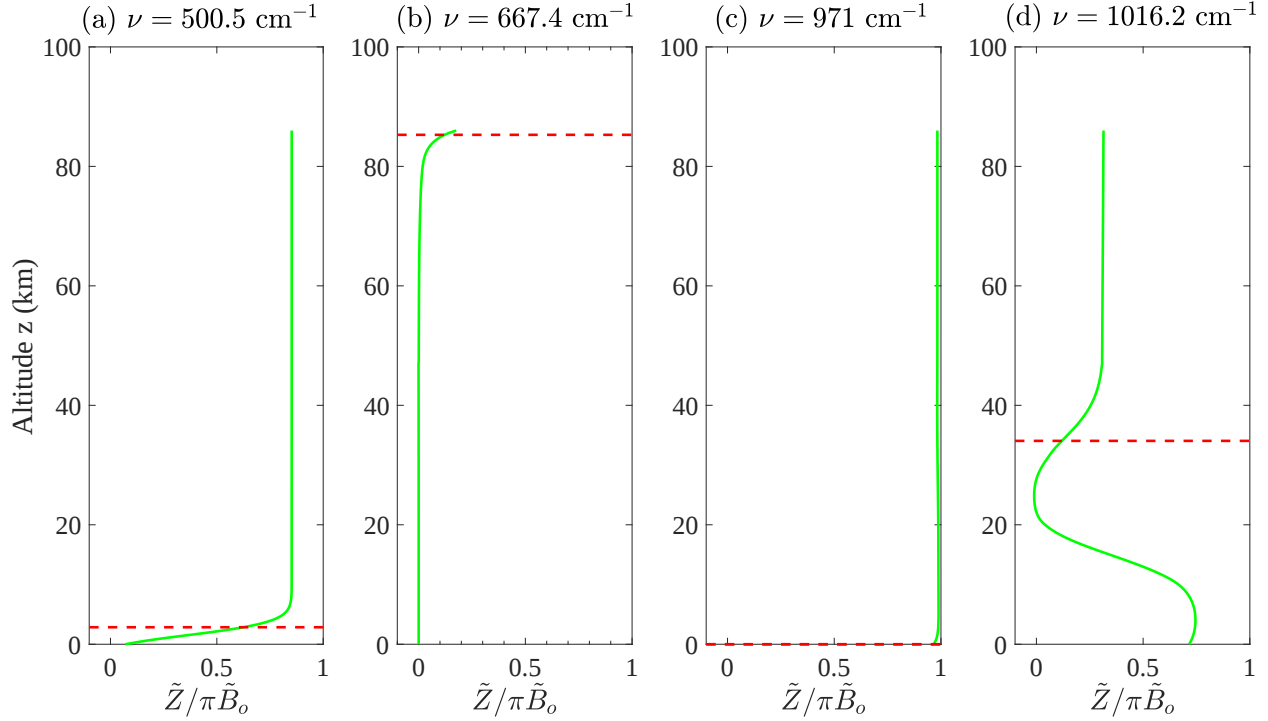
Figure 8: Spectral fluxes \tilde{Z} , like those of Fig. 7, for other representative frequencies, \nu : (a) \tau_{\text{mp}} = 2.30 , z_e = 2.9 \text{ km} , \tilde{B}_o = 134.2 \text{ i.u.} ; (b) \tau_{\text{mp}} = 51687 , z_e = 85.3 \text{ km} , \tilde{B}_o = 131.8 \text{ i.u.} ; (c) \tau_{\text{mp}} = 0.016 , z_e = 0 \text{ km} , \tilde{B}_o = 86.4 \text{ i.u.} ; (d) \tau_{\text{mp}} = 7.11 , z_e = 34.0 \text{ km} , \tilde{B}_o = 79.3 \text{ i.u.} . Here the spectral intensity unit is 1 \text{ i.u.} = 1 \text{ mW m}^{-2} \text{ cm sr}^{-1} .
