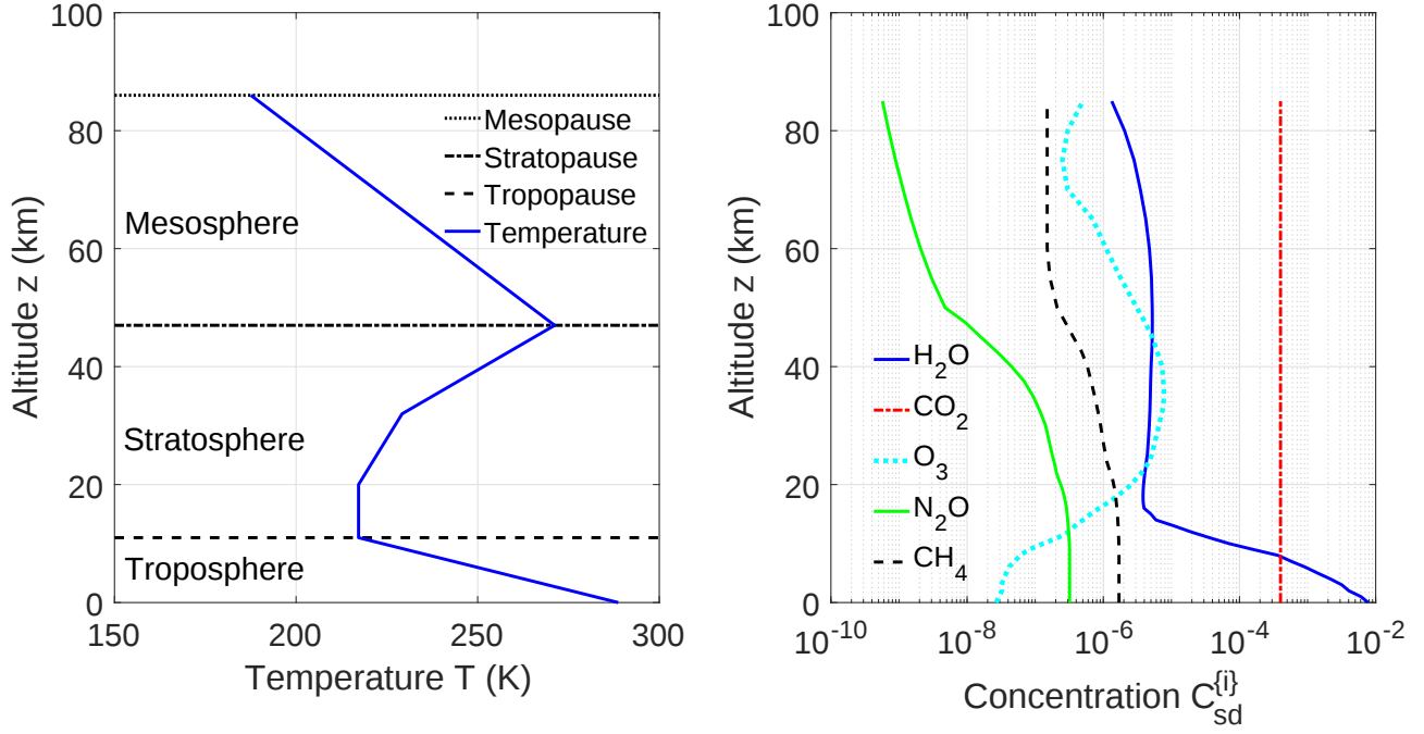
Figure 2: Left. A standard atmospheric temperature profile[15], T = T(z) . The Earth's mean surface temperature is T(0) = 288.7 K . Right. Standard concentrations[16], C_{sd}^{\{i\}} of (3) for greenhouse molecules versus altitude z . At sea level the concentrations are 7750 ppm of H_2O , 1.8 ppm of CH_4 and 0.32 ppm of N_2O . The O_3 concentration peaks at 7.8 ppm at an altitude of 35 km, and the CO_2 concentration was approximated by 400 ppm at all altitudes.
