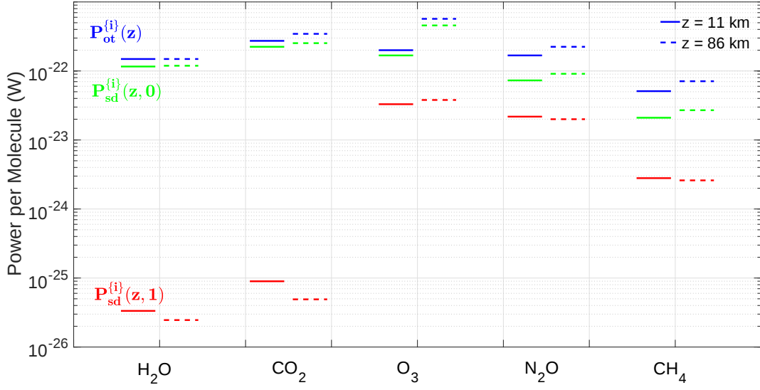
Figure 20: A graphical display of the per-molecule forcing powers of Table 4. At standard column densities the (red) powers, P_{sd}^{\{i\}}(z, 1) , for abundant H_2O and CO_2 are suppressed by four orders of magnitude from their values in the optically thin limit (blue) where the powers are P_{ot}^{\{i\}}(z) . This is due to strong saturation of the absorption bands. The effects of saturation (the difference between the blue and red lines) are much less for the minor gases, O_3 , N_2O and CH_4 . The green lines are the powers per molecule, P_{sd}^{\{i\}}(z, 0) , of the i th greenhouse gas in its low-concentration limit, but when the forcing power is suppressed by other gases at their standard densities. Interference effects (the difference between the blue and green lines) are more pronounced for the minor greenhouse gases, N_2O and CH_4 than for the major greenhouse gases, H_2O , and CO_2 . As one can see from Fig. 6 or Figs. 10 – 12, the strongest bands of O_3 overlap little with those of other greenhouse molecules, which minimizes interference effects.
