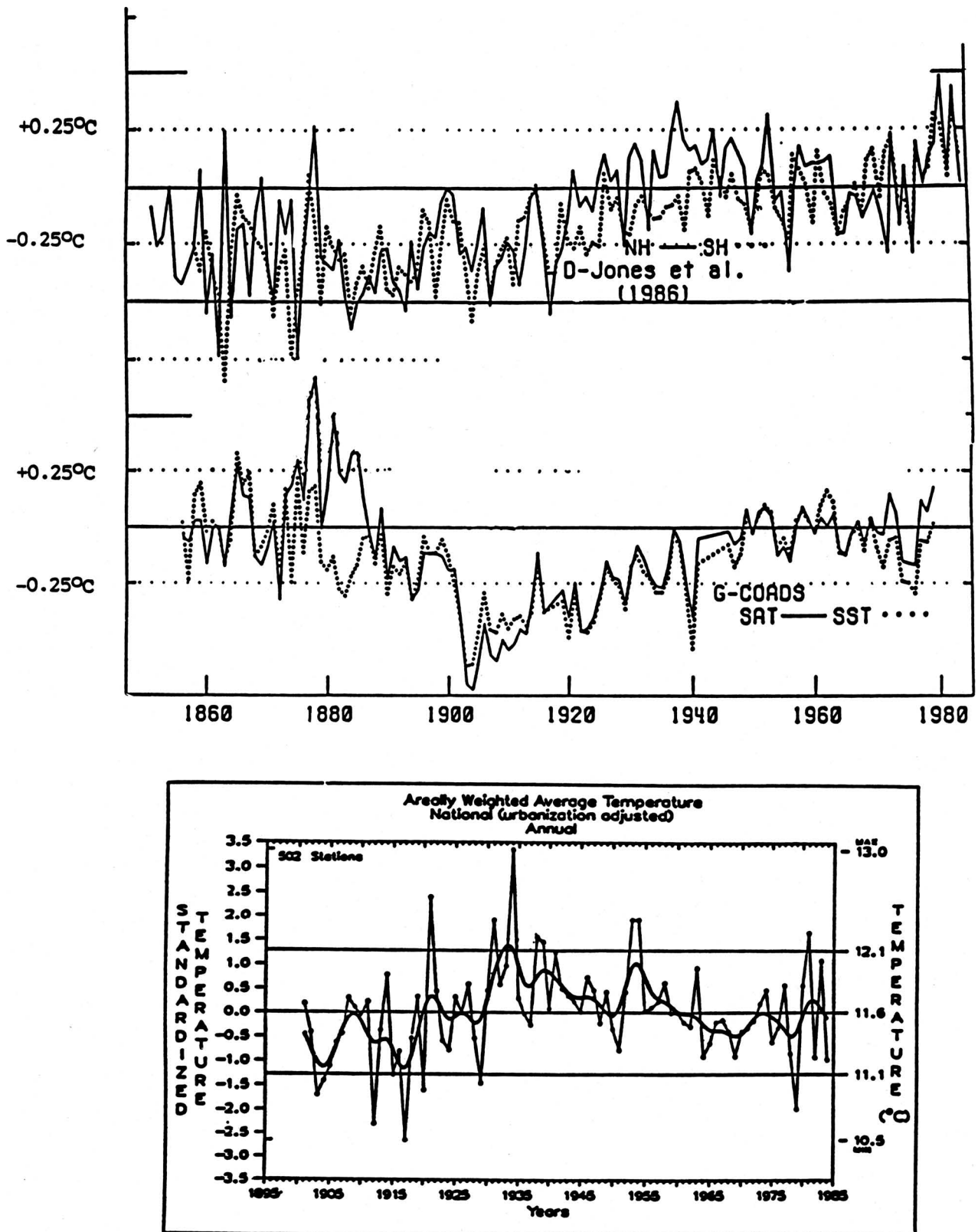
FIG. 2. Annual mean temperature departures (top) from 1951–70 normals derived from station data. The solid curve represents Northern Hemisphere data; the dotted curve represents Southern Hemisphere data. The average between the two tends to be somewhat smoother than either curve. (Reproduced from Ellsaesser et al. 1986, who used analyses from Jones et al. 1986a,b.) Annual mean temperature departures (center) from 1951–70 normal derived from ship data for air temperature (solid line) and sea-surface temperature (dotted line). (Reproduced from Ellsaesser et al. 1986 based on analyses of Slutz, et al. 1985; Ramage 1984; and Folland et al. 1984.) Annual mean temperature (bottom) areally weighted over the contiguous 48 states. The solid curve represents a 9-yr running smoother. (Reproduced from Karl et al. 1988.)
