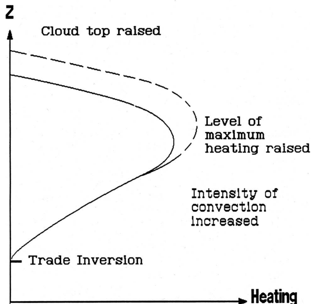
FIG. 8. Schematic illustration of cumulus heating distribution under (solid line) normal conditions, and (dashed line) under conditions of anomalous warming. Warming leads to the following effects: 1) cloud tops are raised leading to dryer detrained air; 2) convective intensity increases which leads to the dryer air being pushed down more effectively; and 3) there is an increase in the height at which there is maximum cumulus heating, thus bypassing more infrared absorbers in the atmosphere.
