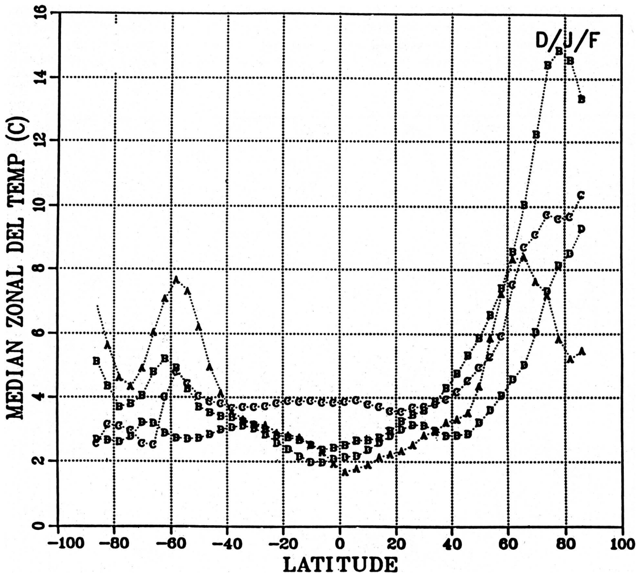
FIG. 3. Superposed medians for four GCMs of the zonal distributions for the predicted change in surface-air temperature due to a doubling of \text{CO}_2 for the period December–February (DJF) (A is the NCAR Community Climate Model; B, GFDL; C, Goddard Institute for Space Studies; and D, Oregon State University). (After Grotch [1988].)
