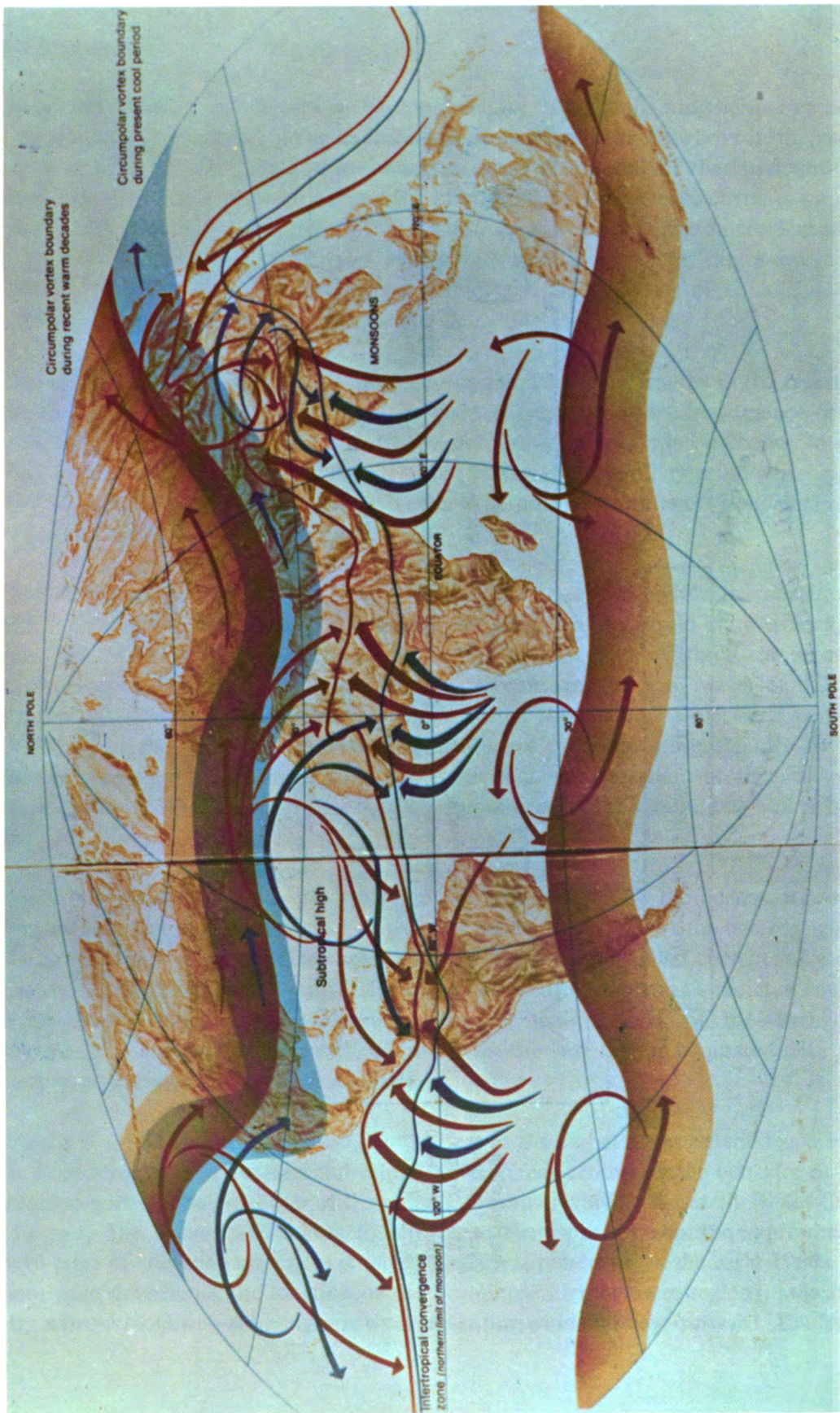
Figure 3. Global Weather Variations
