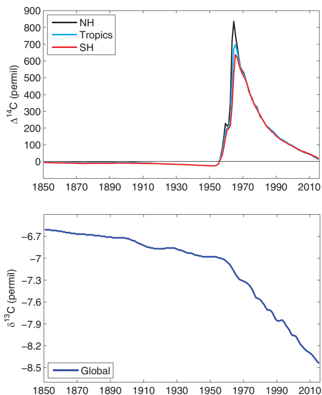
Figure 3. Compiled historical data sets for \Delta^{14}\text{C} (top) and \delta^{13}\text{C} (bottom) from Graven et al. (2017). Annual mean values of \Delta^{14}\text{C} are provided for three zonal bands representing the Northern Hemisphere (30–90°N), the Tropics (30°S to 30°N), and the Southern Hemisphere (30–90°S). Annual mean, global mean values are provided for \delta^{13}\text{C} .
